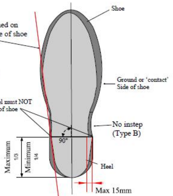
View of bottom of the shoe without 'cut-out' instep
